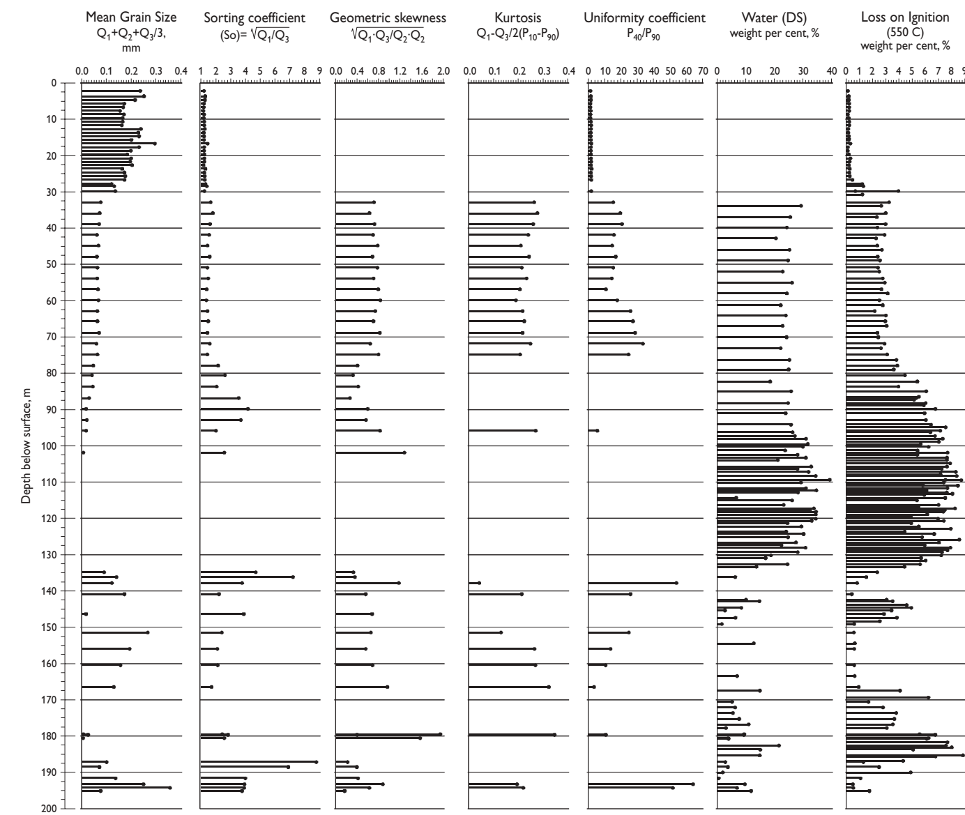
C: Classification of fragmental deposits
