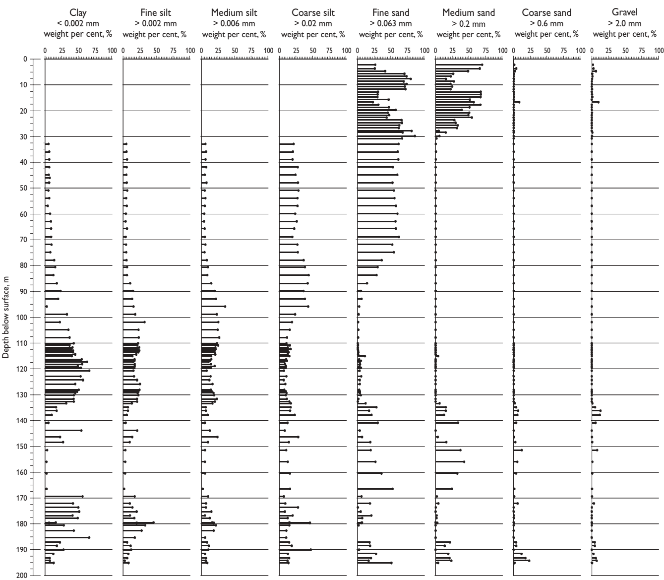
A: Grain size distribution
