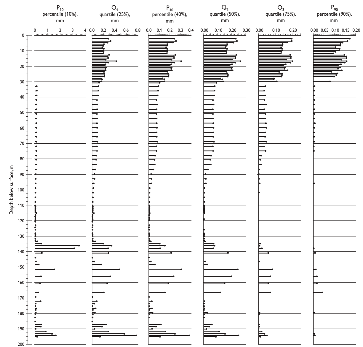
B: Quartiles and percentiles
