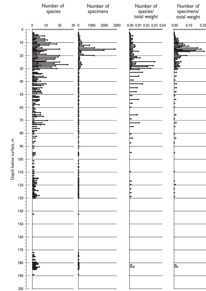
D: Species and specimens diversity
