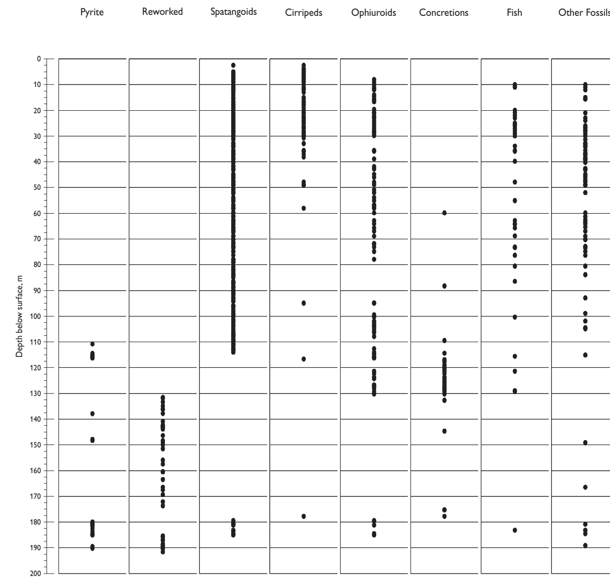
E: Occurrences of minerals, fossils and reworked molluscs
